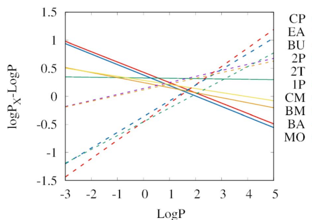
Fig. 4 Extraction efficiencies from water of the individual biobased solvents relative to 1-octanol (log P_x - \log P ). The lines show the linear regressions from Fig. 3. Positive values mean that the solvent exhibits a higher extraction efficiency than 1-octanol. The selected green solvents are abbreviated as cyclopentanol (CP), ethyl acetate (EA), 1-butanol (BU), 2-pentanol (2P), 2-methyl tetrahydrofuran (2T), 1-pentanol (1P), cyclopentyl methyl ether (CM), butyl methyl ether (BM), butyl acetate (BA), and methyl oleate (MO). Some solvents show significantly higher extraction yields than 1-octanol: cyclopentanol, and 1-butanol for hydrophilic solutes (log P < 0.5), as well as cyclopentyl methyl ether and butyl methyl ether for hydrophobic solutes (log P > 2.6). For log P values in the range between 0.5 and 2.6, ethyl acetate and 1-pentanol are the most efficient extraction solvents from water.
