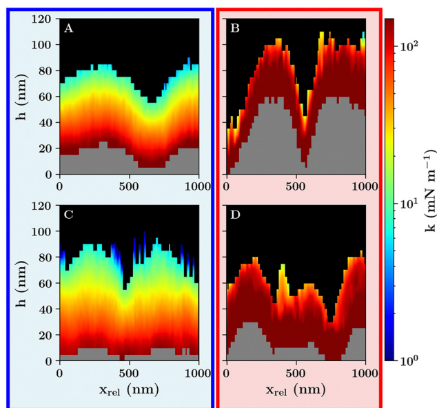
Fig. 10 Example stiffness profiles for monolayers M1 (A) and (B) (C) and (D), below (left) and above the VPTT (right). The black areas indicate a lack of stiffness data because the probe is not in contact with the sample. The grey areas indicate a lack of stiffness data for the set trigger threshold of 4 nN because the sample is not further deformed.
