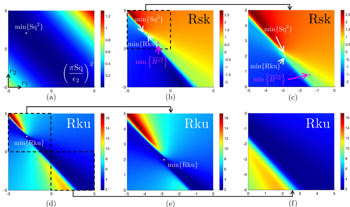
Fig. 7 The analytic result of surface roughness in the (r_1, r_2) parametric space. (a)–(d) Are the scaled (\pi Sq/\epsilon_2)^2 plot, the skewness plot and the kurtosis plot for (r_1, r_2) \in [-5, +5]^2 , respectively. (c) Shows the second quadrant of (b). (e) and (f) Show the second and the fourth quadrants of (d), respectively. The global minima for (\pi Sq/\epsilon_2)^2 > 0 and Rku > 0 are marked with white dots. The \min\{H^{*2}\} surface is marked with a magenta dot. The location and the minimized values are: (a) r_1 = -2.92 , r_2 = +2.08 and \min\{(\pi Sq/\epsilon_2)^2\} = 3.8742 \times 10^{-4} . (d) r_1 = -2.86 , r_2 = +1.98 and \min\{Rku\} = 1.8833 .
