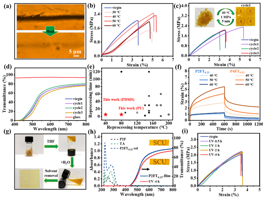
Fig. 2 Physical properties of P2FT 0.25 . (a) Photos of the scratched P2FT 0.25 film treated at 100 °C for 1 h. (b) Stress-strain curves of P2FT 0.25 for different reprocessing temperature. (c) Stress-strain curves of P2FT 0.25 for different recycling cycle. (d) Visible light spectra of glass and P2FT 0.25 film with different recycling cycle. (e) Comparison of P2FT 0.25 and other vitrimers in terms of reprocessing temperature and time. (f) Creep experiment plots of P2FT 0.25 and P4FT 0.25 . (g) Recycling process of P2FT 0.25 (thickness: 170 \mu m). (h) UV-vis spectra of P2F (PDMS-NH 2 and 2-FPBA), TA, P2FT 0.25 solution, P2FT 0.25 film (thickness: 500 \mu m), and P2FT 0.25 film irradiated by UV for 4 h. (i) Stress-strain curves of P2FT 0.25 film irradiated by UV for different time.
