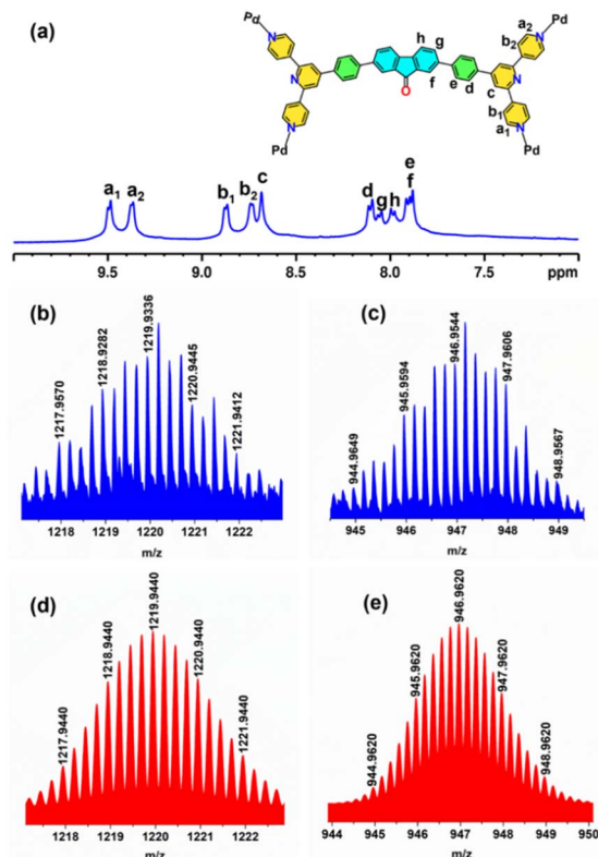
Fig. 1 (a) ^1\text{H} NMR spectrum of trifacial barrel M1 in \text{DMSO}-d_6 at 298 K. (b) Experimental (blue) and (d) theoretical (red) isotopic patterns for the charged fragment [\text{M1}-4\text{PF}_6]^{4+} . (c) Experimental (blue) and (e) theoretical (red) isotopic patterns for the charged fragment [\text{M1}-5\text{PF}_6]^{5+} in ESI-MS recorded in acetonitrile.
