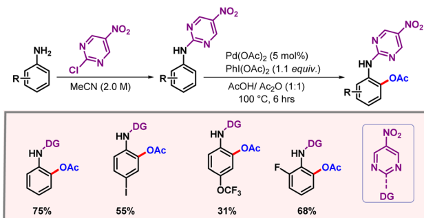
Scheme 9 Pyrimidine enabled ortho -C–H acetoxylation of anilines.
