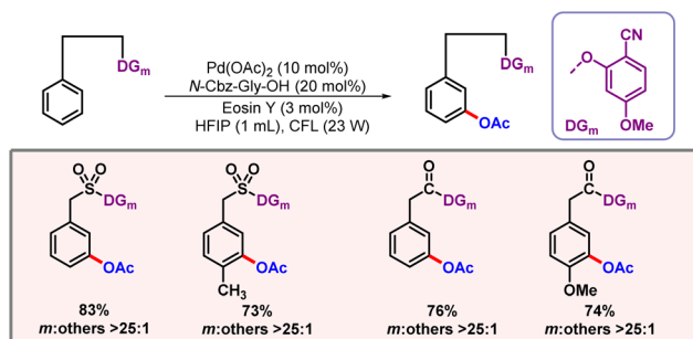
Scheme 55 Photoinduced meta -C–H acetoxylation of arenes.
