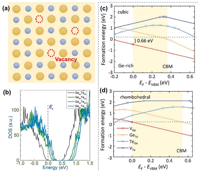
Fig. 8 (a) Schematic view of Ge vacancies in the GeTe matrix. (b) DOS for rhombohedral Ge_{64-x}Te_{64} with different amounts of Ge deficiencies. 128 The formation energy of atomic defects in (c) cubic and (d) rhombohedral GeTe as a function of the relative Fermi-energy under Ge-rich conditions. 129
