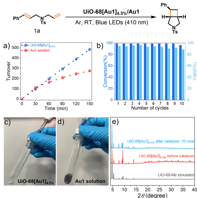
Fig. 5 (a) Product turnovers in the [2 + 2] cycloaddition of 1a to 2a by UiO-68[Au1] _{4.5\%} or Au1 (referring to [Au(C ^N ^N^C)(NHC)]PF _6 ); (b) substrate conversion and product yield in recycling experiments with ten reaction cycles using UiO-68[Au1] _{4.5\%} as the photocatalyst in the given reaction; (c and d) photographs of the photocycloaddition of 1a involving UiO-68[Au1] _{4.5\%} or Au1 , taken after the reaction; (e) PXRD patterns of UiO-68-Me (simulated) and UiO-68[Au1] _{4.5\%} before and after catalysis (measured).
