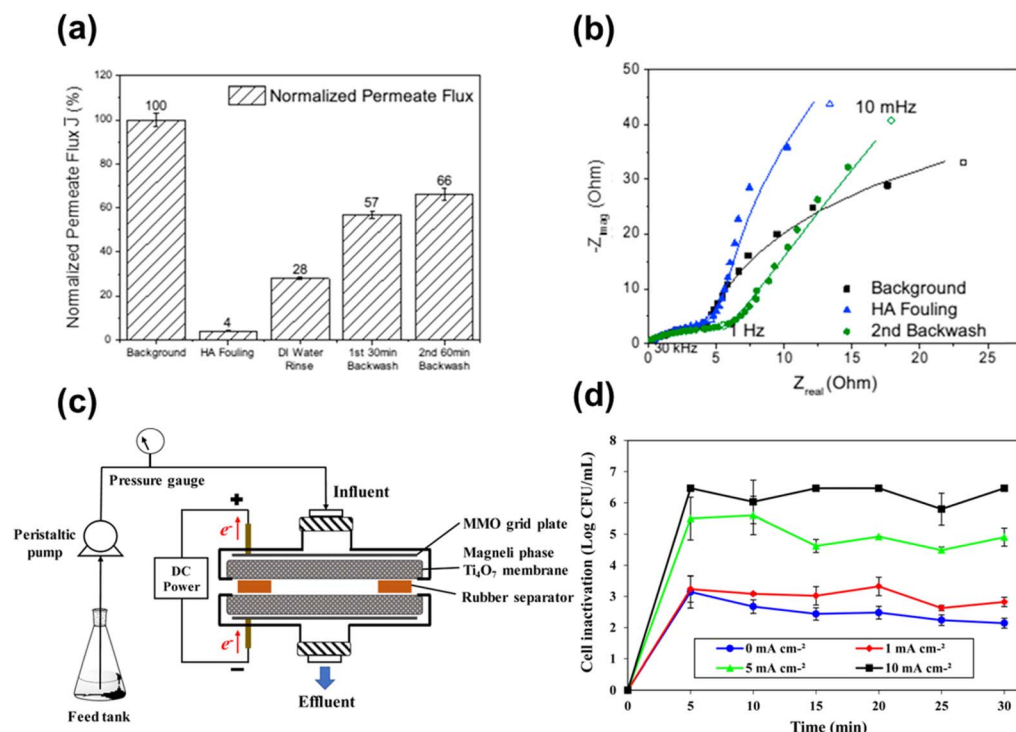
Fig. 18 (a) Normalised permeate flux under different operational conditions for the anodic chemical-free electrochemical regeneration in backwash mode of 150 mg L -1 humic acid fouled REM and (b) electron impedance spectra obtained in the complete frequency range. Reprinted with permission from ref. 124. Copyright 2016, Elsevier. (c) REM system containing \text{Ti}_4\text{O}_7 ceramic membrane design and setup. (d) Effect of different current densities on the removal of E. coli by the \text{Ti}_4\text{O}_7 membrane filtration system. Reprinted with permission from ref. 207. Copyright 2018, Elsevier.
