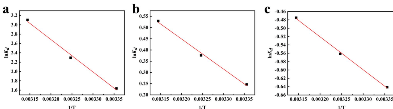
Fig. 8 Thermodynamic model fittings for \text{Pb}^{2+} , \text{Cu}^{2+} , and \text{Cd}^{2+} adsorption by coal gangue and nFeOOH-CG. (a) \text{Pb}^{2+} adsorption thermodynamic fitting plot. (b) \text{Cu}^{2+} adsorption thermodynamic fitting plot. (c) \text{Cd}^{2+} adsorption thermodynamic fitting plot. (Experimental conditions: adsorbent dosage = 5 \text{ g L}^{-1} , initial pH = 4, initial concentration = 100 \text{ mg L}^{-1} , agitation speed = 150 rpm).
