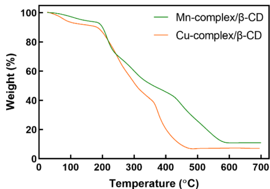
Fig. 4 TGA curves of Mn-complex/β-CD and Cu-complex/β-CD.
