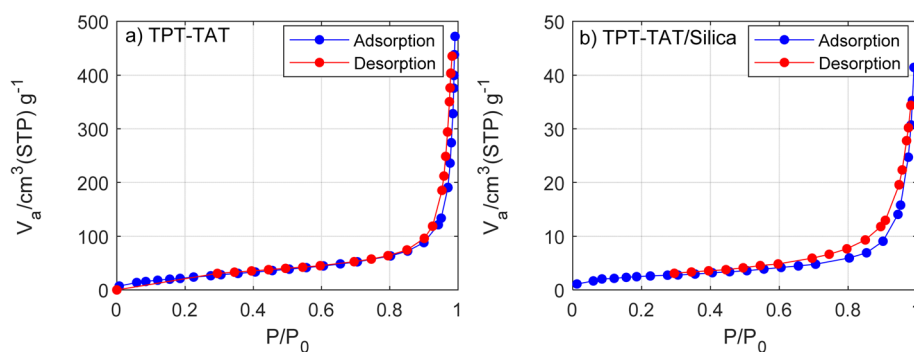
Fig. 5 Adsorption and desorption isotherms of (a) TPT-ATA and (b) TPT-TAT/silica. Adsorptive N_2 and adsorption temperature at 77 K.
