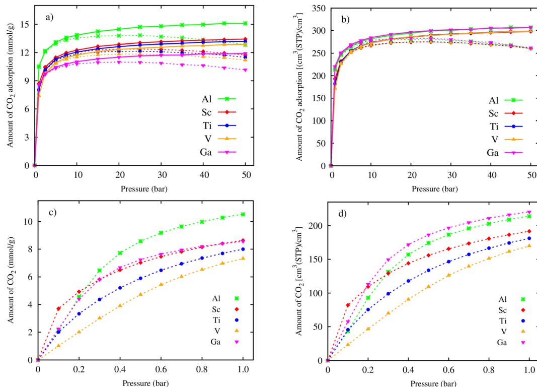
Fig. 3 Excess (dashed lines) and absolute (solid lines) \text{CO}_2 adsorption isotherms of MIL-88A(M), where M = Al, Ga, Sc, Ti, and V: (a) gravimetric uptake and (b) volumetric uptake for pressures of up to 50 bar. Zoom-in for gravimetric (c) and volumetric (d) \text{CO}_2 adsorption isotherms at low pressures (0–1.0 bar).
