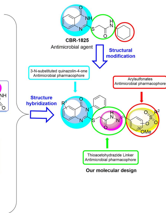
Fig. 1 Marketed drugs containing quinazolinone, hydrazide–hydrazone, or sulfonate motifs along with our molecular design.
