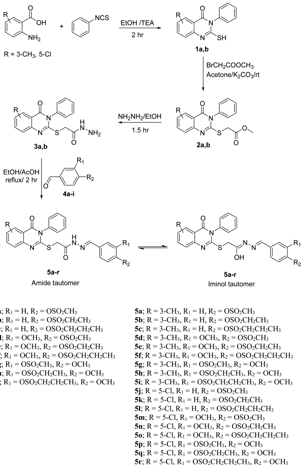
Scheme 1 The synthetic route toward quinazolinone-sulfonate conjugates with their tautomers 5a-r.
