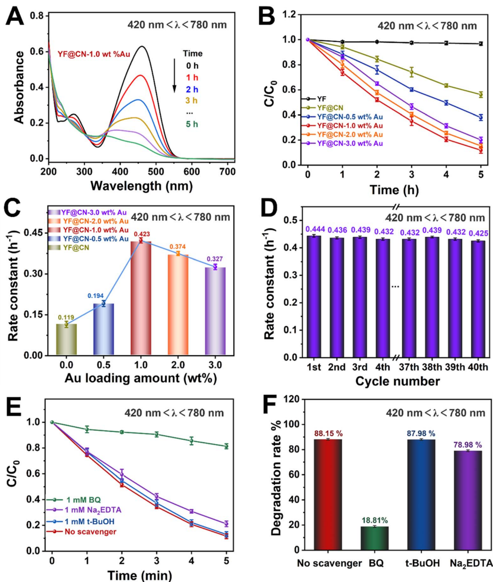
Fig. 4 The MO photodegradation activity under visible light (420 nm < λ < 780 nm) irradiation: (A) absorption spectra of MO photodegradation for YF@CN-1.0 wt% Au after different irradiation time; (B) the MO photodegradation over YF, YF@CN and YF@CN- x wt% Au and (C) the corresponding rate constants; (D) the rate constants of YF@CN-1.0 wt% Au during 40 consecutive cycles, each lasting 5 h; (E) effects of three different scavengers on the MO degradation over YF@CN-1.0 wt% Au and (F) the corresponding MO degradation rates after 5 h.
