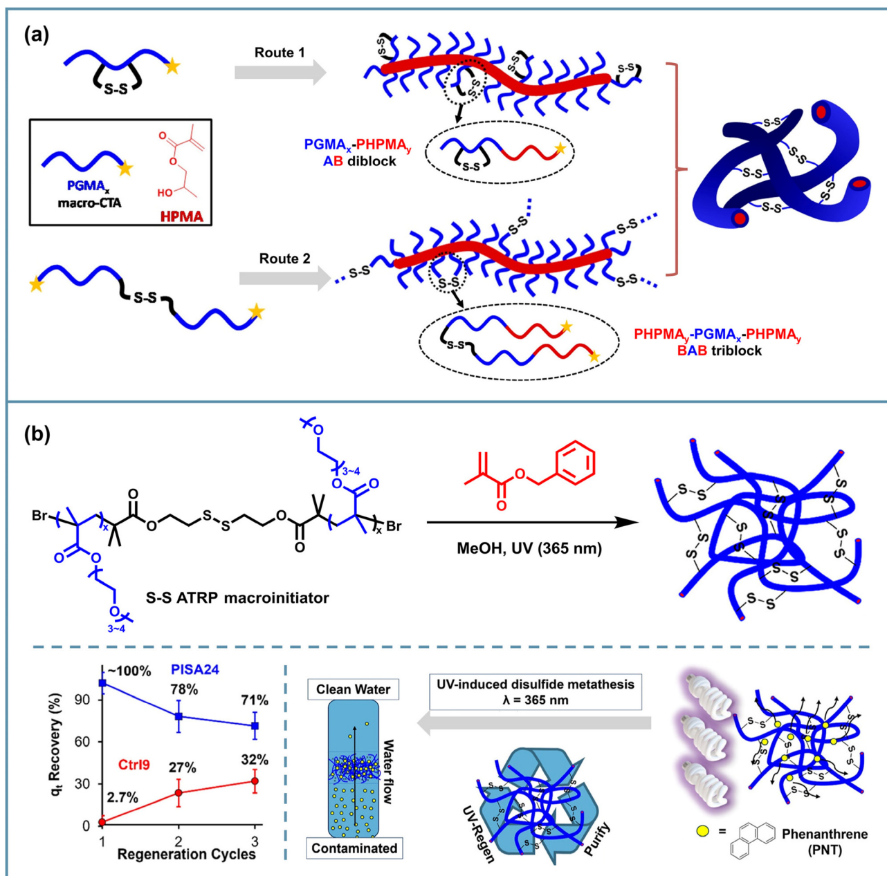
Fig. 4 Schematic illustration of disulfide-crosslinked PISA worm gels: (a) reductant-responsive worm gels based on PGMA-HPMA using the disulfide-based methacrylic comonomer DSDMA or a GMA45-S-S-GMA45 disulfide-based difunctional macro-CTA. Adapted with permission from ref. 69. Copyright 2015 American Chemical Society. (b) UV-responsive worm gels based on PBMA- b -POEGMA- b -PBMA and PGlyMA- b -POEGMA- b -PGlyMA, and the overall recovery of the adsorption capacity ( q_t ) for both PISA24 (PBMA- b -POEGMA-S-S-POEGMA- b -PBMA) and Ctrl9 (PBMA- b -POEGMA- b -PBMA) calculated based on the obtained kinetic data for three UV-regeneration cycles. Adapted with permission from ref. 71. Copyright 2024 American Chemical Society.
