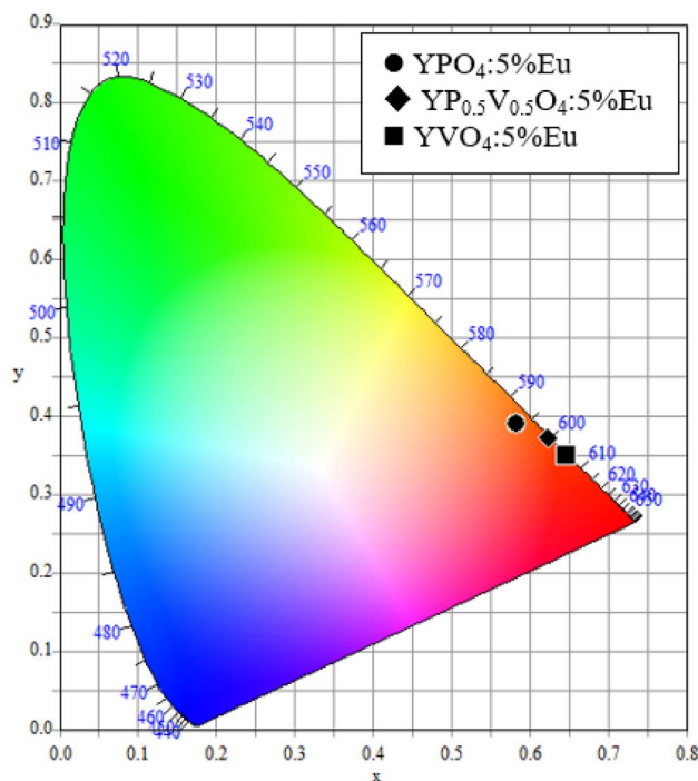
Fig. 9 CIE chromaticity diagram for emission spectra of \text{YP}_{(1-x)}\text{V}_x\text{O}_4\cdot 5\% \text{Eu}^{3+} ( x = 0, 0.5, 1 ).
