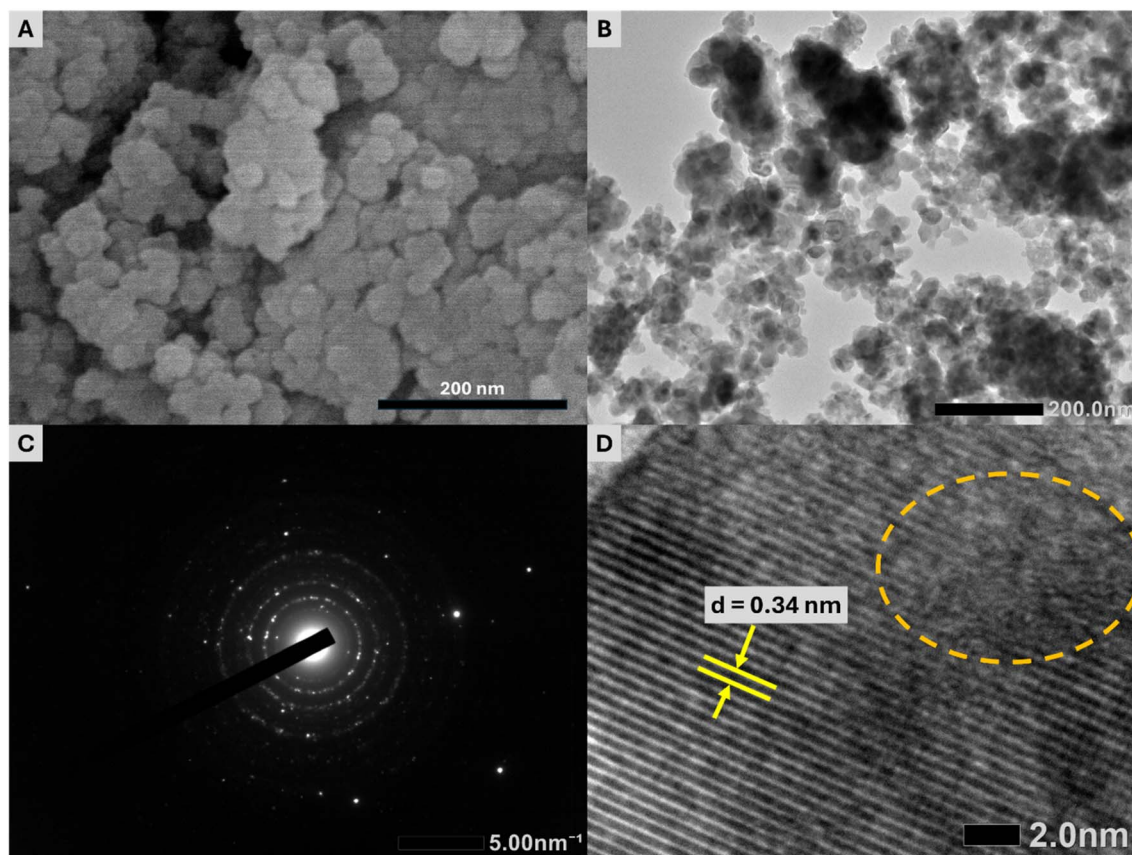
Fig. 3 (A) SEM, (B) TEM, (C) SAED, and (D) HR-TEM images of the \text{Y}(\text{P}_{0.5}\text{V}_{0.5})\text{O}_4\text{:}5\% \text{Eu} sample.
