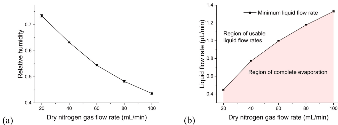
Fig. 4 Experimentally determined (a) relative humidity and (b) liquid flow rate for various dry nitrogen gas flow rates range from 20 to 100 mL min -1 at 30 °C. The liquid flow rate is 2 \mu L min -1 .
