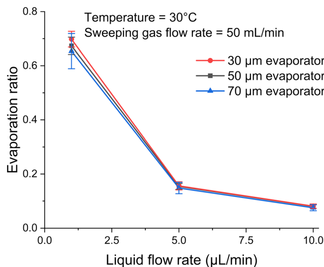
Fig. 7 Deionized water evaporation versus liquid flow rate from 1 to 10 \mu\text{L min}^{-1} for three different pore diameters under the condition of 30 °C and 50 \text{mL min}^{-1} of sweeping gas flow rate.
