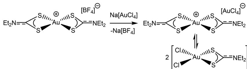
Scheme 4 Regeneration of the [\text{AuCl}_2(\text{Et}_2\text{dtc})]/[\text{Au}(\text{Et}_2\text{dtc})_2]^+ mixture by metathesizing stable [\text{Au}(\text{Et}_2\text{dtc})_2][\text{BF}_4] with \text{Na}[\text{AuCl}_4] .
