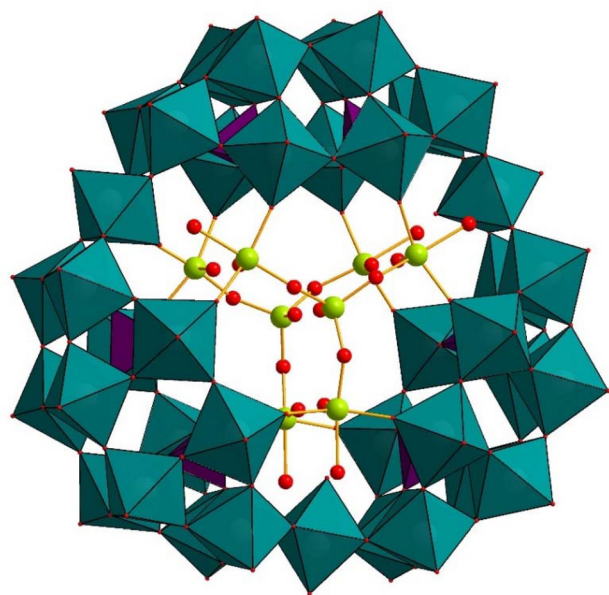
Fig. 11 Combined polyhedral/ball-and-stick representation of [\text{Rb}_3\text{C}\{\text{V}^{\text{IV}}\text{V}^{\text{IV}}\text{O}_7(\text{H}_2\text{O})_6\}_2\{\text{H}_6\text{P}_6\text{W}_{39}\text{O}_{147}(\text{H}_2\text{O})_3\}]^{15-} . Color code: \text{WO}_6 octahedra (green), \text{PO}_4 tetrahedra (pink), O (red), V (yellow). 93
