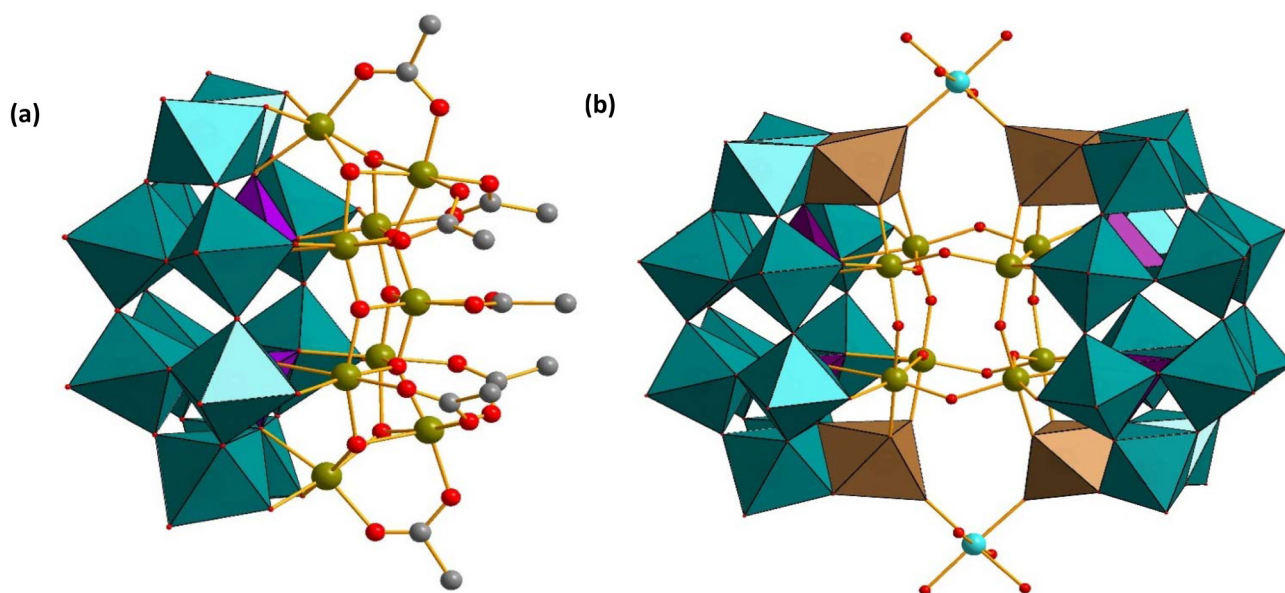
Fig. 4 Combined polyhedral/ball-and-stick representations of (a) [\text{H}_4\text{P}_2\text{W}_{12}\text{Fe}_9\text{O}_{56}(\text{CH}_3\text{COO})_7]^{12-} ( \text{Fe}_9\text{P}_2\text{W}_{12} ), and (b) \{[\text{M}(\text{H}_2\text{O})_4]_2(\text{H}_{12}\text{P}_4\text{W}_{28}\text{Fe}_8\text{O}_{120})\}^{12-} ( \text{M} = \text{Co}^{2+}, \text{Mn}^{2+}, \text{Ni}^{2+} ). Color code: \text{WO}_6 octahedra (green and brown), \text{PO}_4 tetrahedra (pink), Fe (green), M (turquoise), O (red), C (grey). H atoms on carbon have been omitted for clarity. 58,59
