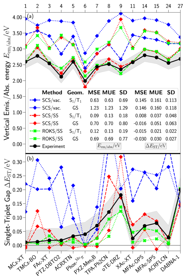
Fig. 7 Experimental (black) and calculated emission energies E_{em} (a) and singlet–triplet gaps \Delta E_{ST} (b) for subset A of the STGABS27 benchmark set. The calculated values are given either at the excited state ( S_1/T_1 ) geometries optimized with UKS/ROKS/PCM using the OT-LC- \omega PBE functional (dashed lines) or at the ground state (GS) geometries optimized with PBEh-3c (dotted lines) from ref. 30. Results are shown for SCS-ADC(2)/vacuum (blue), SCS-ADC(2)/SS-COSMO (red), and ROKS/PCM (green) with the OT- \omega B97M-V functional all using the def2-SVP basis set. All calculations of \Delta E_{ST} employ a dielectric constant of \epsilon = 3.0 , while calculations of E_{em} employ system-specific values for \epsilon and the refractive index n dependent on the experimental measurement. Connecting lines between individual datapoints serve only to guide the readers eye. The target error margin corresponding to chemical accuracy ( \approx \pm 0.05 eV) for \Delta E_{ST} and conservative experimental errors of \pm 0.2 eV for the E_{em} is marked by grey bands around the experimental values. MSE and MUE values for subset A of the STGABS27 are tabulated.
