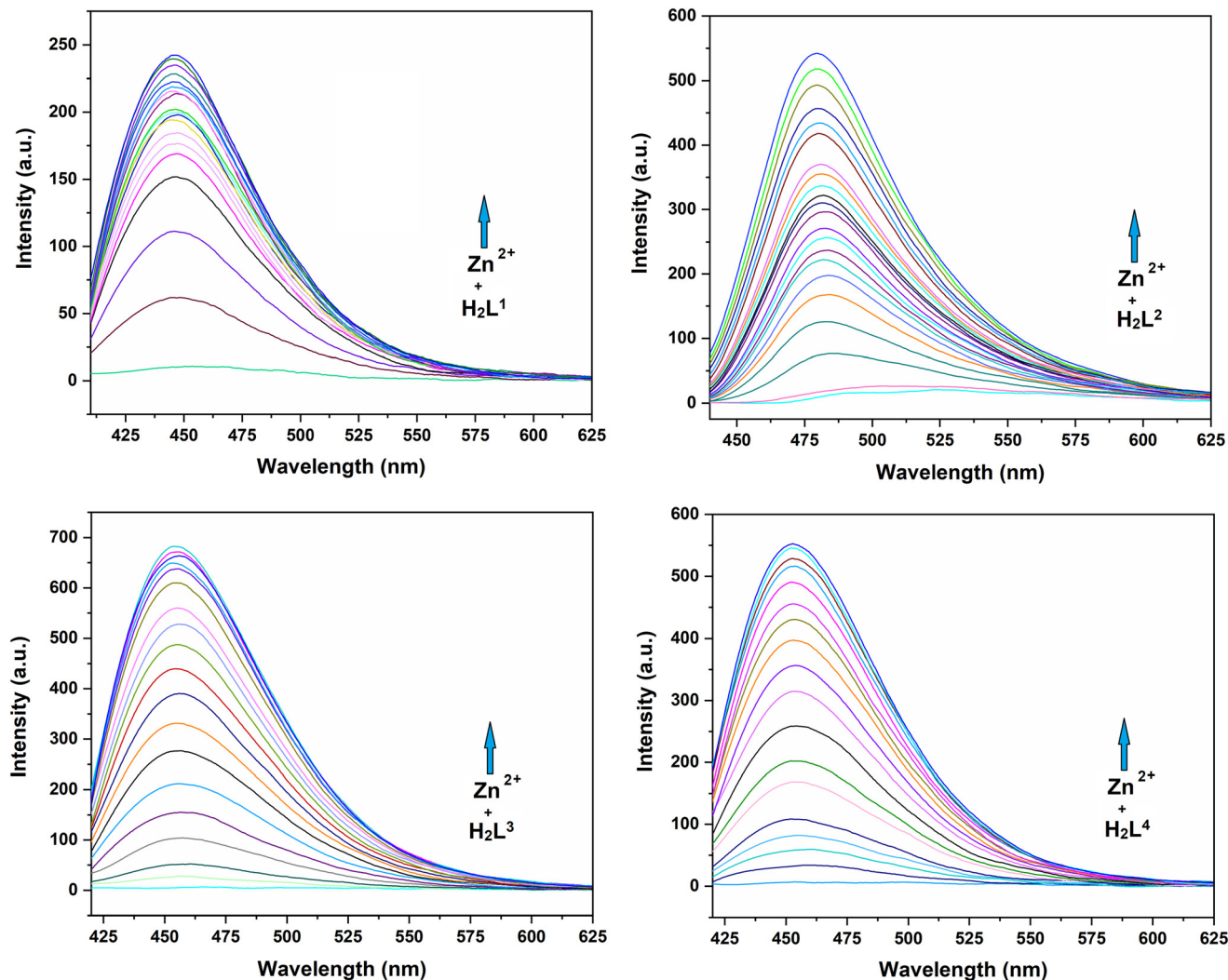
Fig. 11 Emission spectra of 10^{-3} M Schiff base ligands \text{H}_2\text{L}^1 (excitation 397 nm, 446 nm) or \text{H}_2\text{L}^2 (excitation 419 nm, emission 479 nm) or \text{H}_2\text{L}^3 (excitation 397 nm, emission 454 nm) or \text{H}_2\text{L}^4 (excitation 397 nm, 453 nm) in the presence of increasing concentration of free \text{Zn}^{2+} ions at room temperature.
