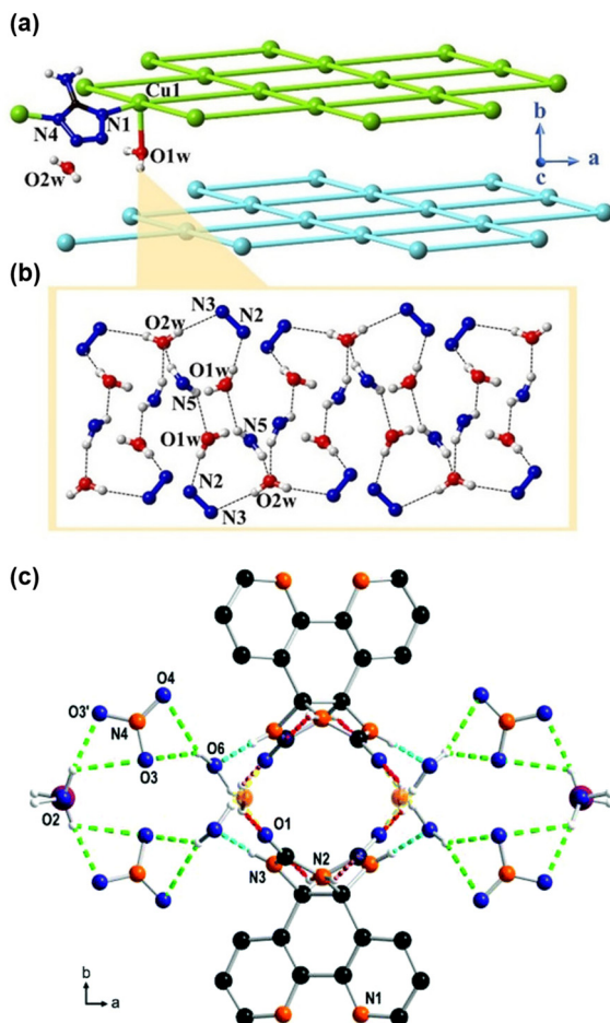
Fig. 6 (a) The stacking sq1 networks for complex 1 , among that atz - ligands can be considered as sticks. (b) The coordinated water molecules O1w and free water molecules O2w are linked into 1D hydrogen transport channel by hydrogen bonds with atz - ligands. Reproduced with permission from ref. 68, Copyright 2021, Wiley, VCH. (c) Ligand NH...O (red) ligand donor-acceptor bonds are responsible for the formation of channels along [001]. In addition ligand NH...O water (bluish), water OH...O (green) and water OH...O ligand (yellow) hydrogen donor-acceptor bonds are observed (color code: N = orange, O = blue and Cu = purple). Reproduced with permission from ref. 69, Copyright 2017, Royal Society of Chemistry.
