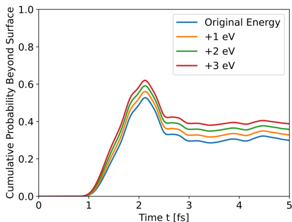
Fig. 4 Wave propagation of holes through the ^*\text{O} slab using different initial total energies.
