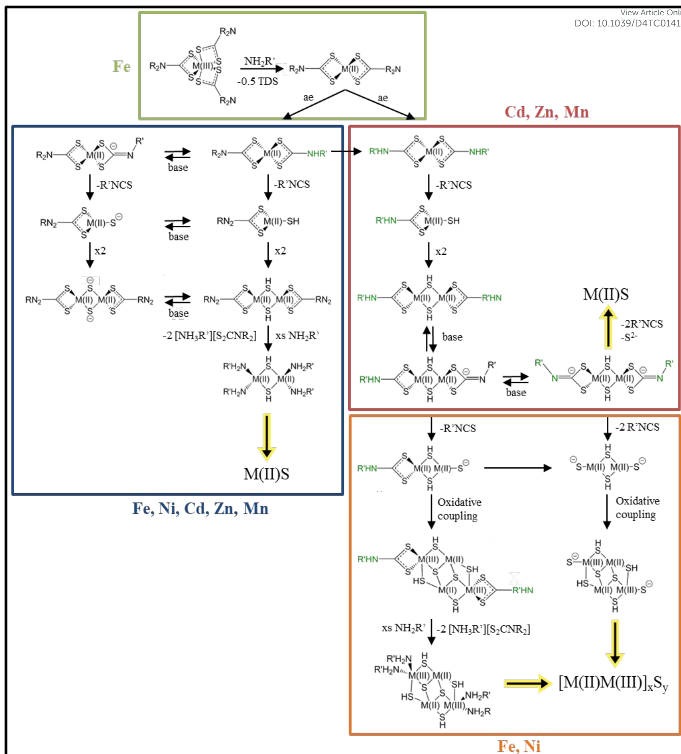
Figure 6. Possible reactions of metal dithiocarbamate complexes in a primary amine solvent. Summarized reactions from Ref. 111, 112, 113, 114, 116. For simplicity the possible coordinated primary amine molecules are left out.
