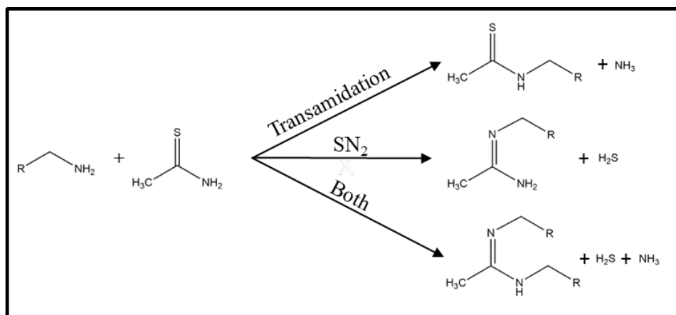
Figure 2. Reactions of a primary amine with thioacetamide. Adapted with permission from Ref. 61. Copyright 1971 IOP.
