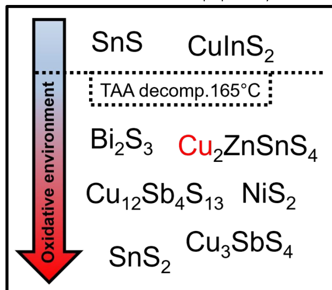
Figure 3. Scheme of synthesized materials with thioacetamide (TAA) as sulfur source and oleylamine as solvent. Materials synthesized at higher temperatures as the decomposition temperature of TAA (165°C) have the most stable oxidation state. Copper in Cu 2 ZnSnS 4 (CZTS) is stated in red because Cu(I) is not the most stable oxidation state, but in the synthesis of CZTS Cu(II) is used as precursor, whereas Sn has its most stable oxidation state (+IV). Materials synthesized at lower temperature than the decomposition temperature of TAA can have an oxidation state different than the most stable one.
