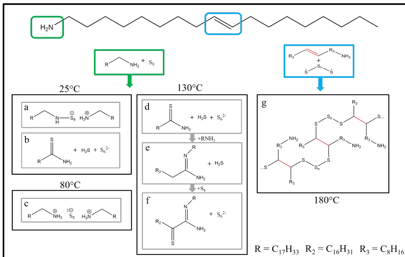
Figure 1. Molecule structure for oleylamine. Depicted in the green box reaction of elemental sulfur with a primary amine functional group. a), b) reaction at 25°C reported in Ref. 31 c) reaction at 80°C reported in Ref. 35 d), e), f) reaction at 130°C reported in Ref. 39. Depicted in the blue box reaction of elemental sulfur with the double bond in oleylamine. g) polymerization reaction at 180°C reported from Ref. 36.
