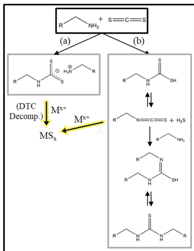
Figure 7. Reactions of carbon disulfide with a primary amine and decomposition reaction into the corresponding metal sulfides. a) reaction reported in Ref. 120 b) reaction reported in Ref. 121
