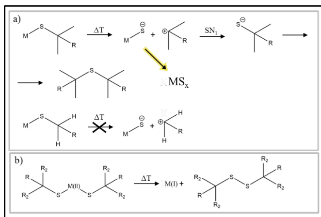
Figure 4. a) thermal decomposition of thiolates and formation of MS_x nanomaterials. Figure adapted from Ref. 79 under Creative Commons Attribution licence CC BY 4.0 b) redox reaction of thiolates and metals reported in Ref. 86
