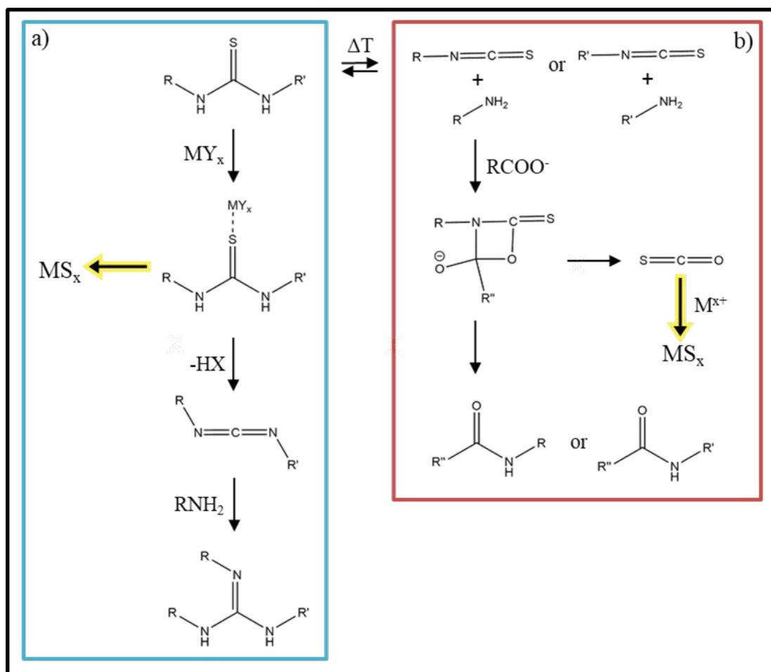
Figure 9. a) The decomposition reaction of substituted thioureas into metal sulfides. Adapted with permission from Ref. 132. Copyright 2023 American Chemistry Society. b) The decomposition reaction into metal sulfides from thioureas at higher temperatures with equilibrium on the isothiocyanate side. Figure adapted from Refs. 133, 134.
