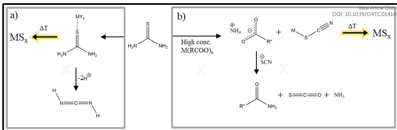
Figure 8. a) decomposition reaction of thiourea into metals sulfides b) decomposition reaction of thiourea with metal carboxylates into metal sulfide materials. Figure adapted from Ref. 128 under Creative Commons Attribution licence CC BC 4.0.
