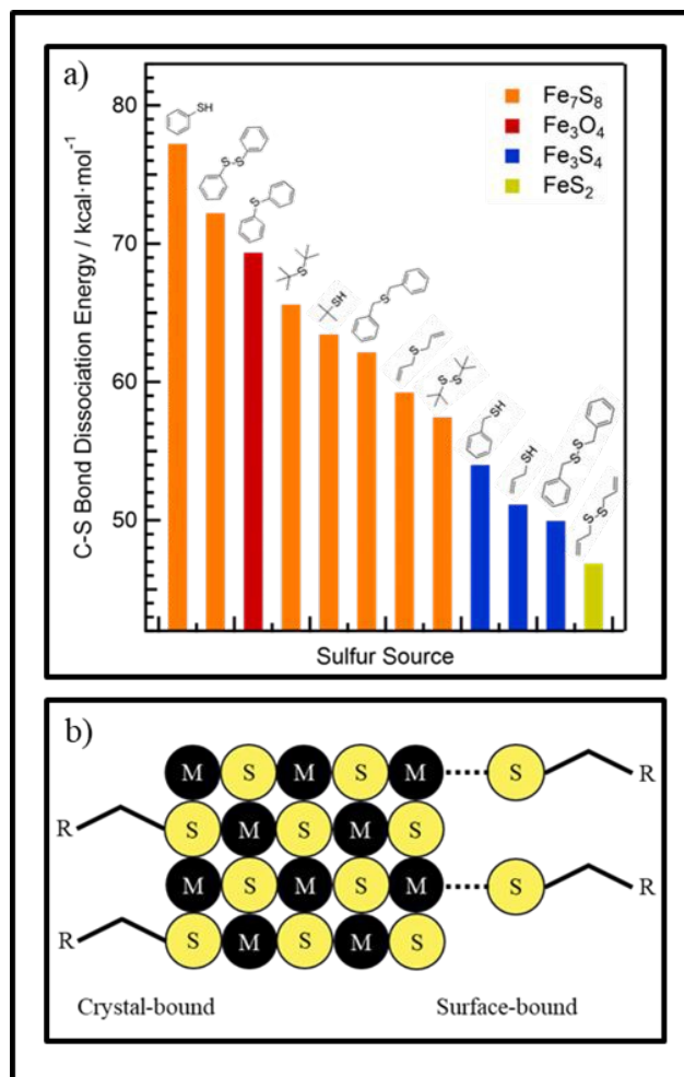
Figure 5. a) reactivity of different sulfur precursors vs. the carbon-sulfur dissociation energy and their products in iron sulfide synthesis. Adapted with permission from Ref. 89. Copyright 2017 American Chemistry Society. b) schematic picture of crystal bound and surface bound thiols. Adapted with permission from Ref. 90. Copyright 2014 American Chemistry Society.
