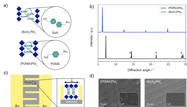
Fig. 1 (a) Schematic of RP (top) and DJ (bottom) phases in this study with the corresponding (BzA, PDMA) spacer structures (cyan) and different alignments of the adjacent inorganic layers (blue). (b) X-ray diffraction patterns of (\text{BzA})_2\text{PbI}_4 (blue) and (\text{PDMA})\text{PbI}_4 (black). Here * corresponds to higher-order ( h00 ) reflections. 24–28 UV-vis absorption spectra of the films are shown in Fig. S1 (ESI†) with XRD patterns showing comparable structures of the materials in films and devices (ESI†). (c) Schematic representation of the electrode substrate (quartz) used for electrical measurements. Inset: Graphic illustration of a DJ perovskite placed between two electrodes. (d) SEM images of (\text{PDMA})\text{PbI}_4 and (\text{BzA})_2\text{PbI}_4 thin films deposited on the substrates with interdigitated contacts (5 \mu\text{m} wide gold fingers are visible in the image). Insets represent the SEM images of the films at higher magnification (the corresponding scale bars are shown on the images).
