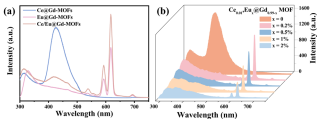
Fig. 2 (a) Emission spectra of Ce@Gd-MOFs, Eu@Gd-MOFs and Ce/Eu@Gd-MOFs, and (b) emission spectra of Ce/Eu@Gd-MOFs ( \lambda_{\text{ex}} = 260 \text{ nm} ).
