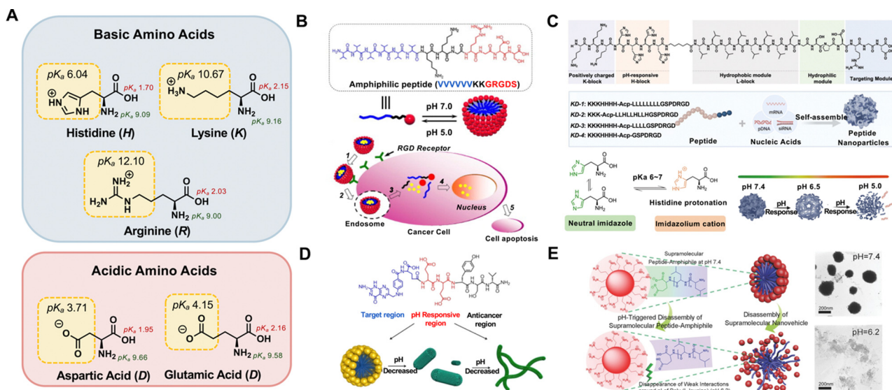
Fig. 2 (A) Structures of common basic and acidic amino acids, with their R-group side chain \text{pKa} values highlighted and drawn in their charged configuration. The \text{pKa} for N- and C-terminal groups are also shown for reference. (B) Schematic illustration of a pH-responsive micelle prepared from an amphiphilic peptide that assembles and disassembles to release anti-tumor drugs within cancer cells. Figure adapted from ref. 57 with permission from Elsevier © 2014. (C) Peptide designed to form pH-sensitive nanoparticles in complexation with nucleic acid payloads. The protonation equilibria and tautomeric forms of the imidazole side chain of histidine offer a pH triggered decomposition of the nanoparticles. Figure adapted from ref. 58 with permission from Royal Society of Chemistry © 2023. (D) Peptide sequence of prodrug FA-EEYSV-NH 2 and its properties pH-responsive assembled nanostructure. Figure adapted from ref. 59 with permission from American Chemical Society © 2021. (E) Scheme depicting the pH-responsive disassembly of complexed supramolecular amphiphiles, with TEM images showing the nanostructure at pH 7.4 and 6.2. Figure adapted from ref. 60 with permission from John Wiley and Sons © 2013.
