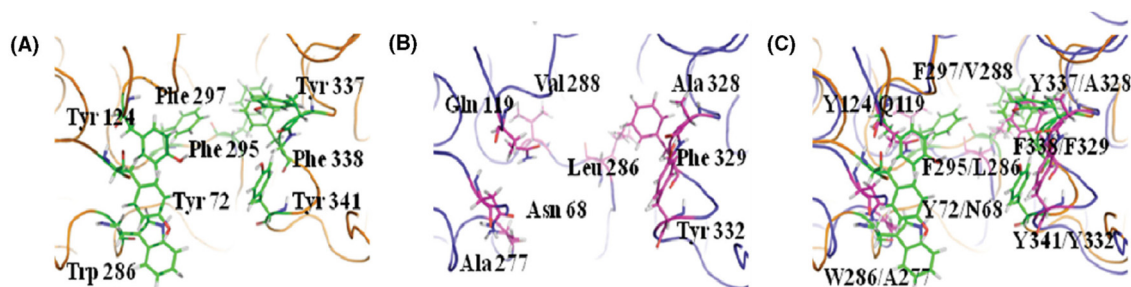
Fig. 3 The residues in the gorge of (A) AChE, (B) BChE, and (C) superimposing of the gating residues in AChE and BChE. Adapted with permission from ref. 79. Copyright 2011 American Chemical Society.
