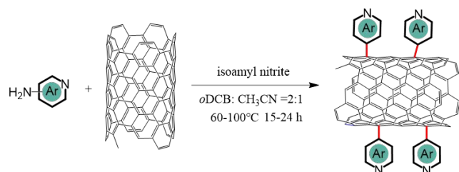
Scheme 1 Synthesis of N-CNTs
