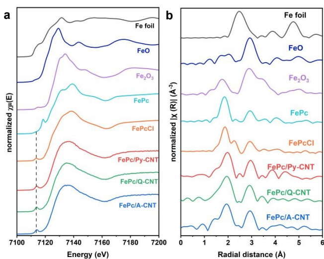
Fig. 2(a) Fe K-edge XANES spectra of as prepared FePc/N-CNTs in comparison with Fe foil, FeO, Fe 2 O 3 , Fe(II)Pc, and Fe(III)PcCl; (b) Fourier Transform (phase-corrected) of FePc/N-CNTs, Fe foil, FeO, Fe 2 O 3 , Fe(II)Pc, and Fe(III)PcCl
