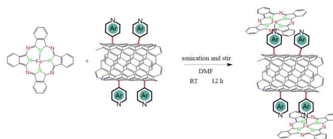
Scheme 2 Synthesis of FePc/N-CNTs
