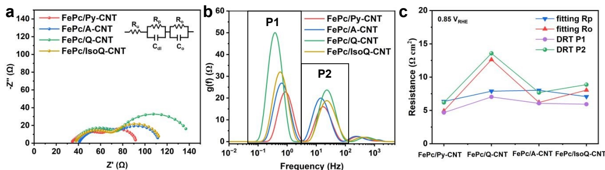
Fig. 5 (a) Electrochemical impedance of FePc/N-CNTs was collected at 0.85 V_{RHE} in a frequency range of 0.1 Hz to 1 M Hz, in oxygen-saturated 0.1 M KOH at a rotational rate of 1600 rpm. The results of the electrochemical impedance spectroscopy fitting with the equivalent circuit are detailed in the supporting information. R_p : polarization resistance and R_o : the oxygen transport resistance. (b) DRT results from EIS spectra. (c) Corresponding calculated resistances from the equivalent circuit fitting and DRT analysis.
