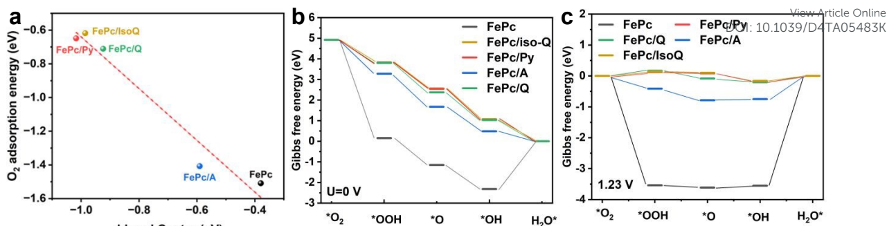
Fig. 6 (a) the correlation between the d-band center and the oxygen adsorption energy (b) Free energy diagram at 0 V for ORR of FePc and FePc/N-heterocycles, with a single-site mechanism. (c) Free energy diagram at 1.23 V for ORR of FePc and FePc/N-heterocycles.
