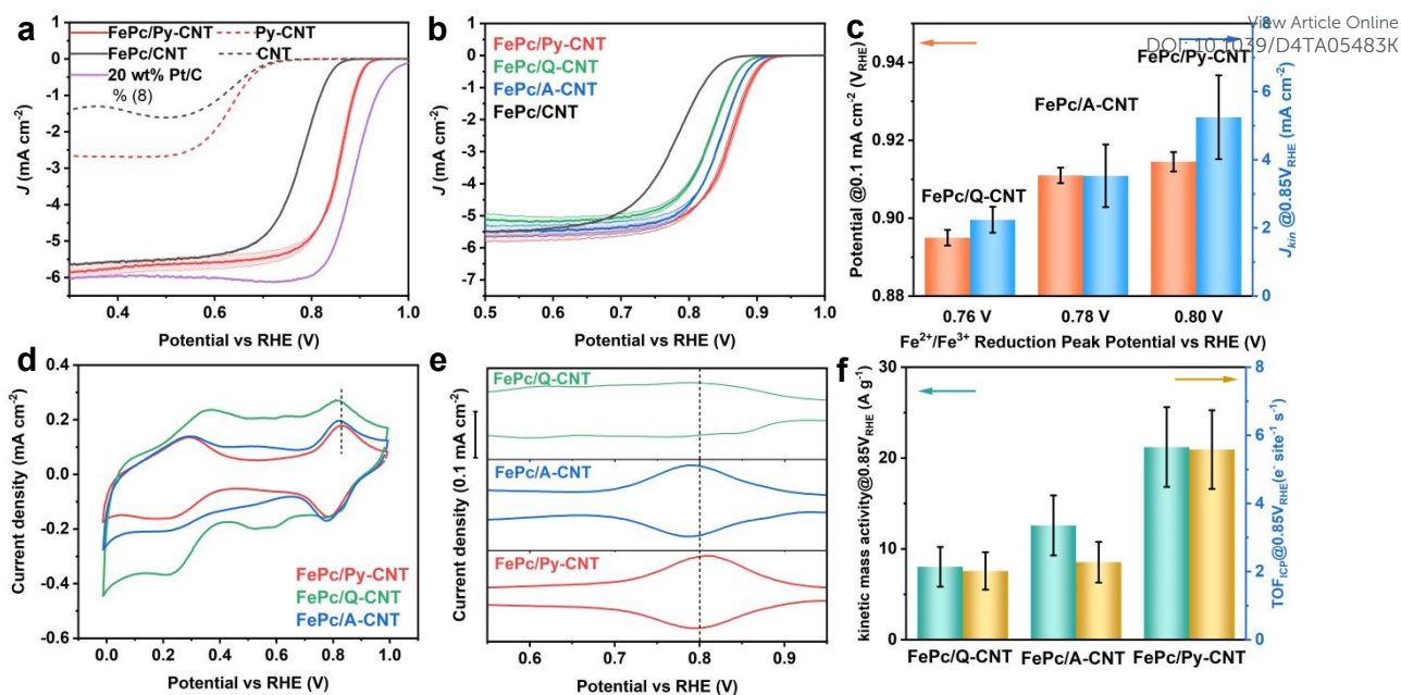
Fig. 3 All the RDE data of FePc/N-CNT, CNT, N-CNT, and 20 wt% Pt/C was collected at room temperature (25 °C) with a Hg/HgO reference electrode and graphite rod counter electrode in 0.1 M KOH. (a) and (b) Cathodic LSV curves obtained by subtracting N 2 -saturated LSV from the O 2 -saturated result (with a rotation rate of 1600 rpm recorded at 10 mV s -1 ). Error bars represent the standard deviation from three separate measurements. (c) Comparison of onset potential (potential @0.1 mA cm -2 ) and kinetic current density @0.85 VRHE. (d) CV N 2 -saturated, in static conditions with a scan rate of 100 mV/s. (e) SWV was obtained in N 2 -saturated, in static conditions, with a frequency of 2 Hz, with 4 mV steps, and a modulation amplitude of 20 mV. (f) Comparison of kinetic mass activity at 0.85 VRHE and turnover frequency at 0.85 VRHE (active site density was calculated based on ICP results).
