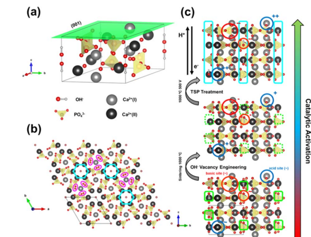
Scheme 1 Structure of HAP as a catalyst. (a) HAP unit cell P6_3/m . (b) (001) crystallographic plane observed from the c -axis direction. The OH - channels and the Ca(l) 6-fold coordination are highlighted. (c) Structural changes and lattice refinement strategies adopted to achieve the catalytic activation of HAP.
