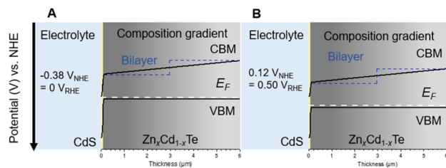
Fig. 8 Expected band diagrams for the cases of the bilayer structure and the composition gradient structure of ZnTe and CdTe at (A) 0 V_{\text{RHE}} and (B) 0.5 V_{\text{RHE}} .
