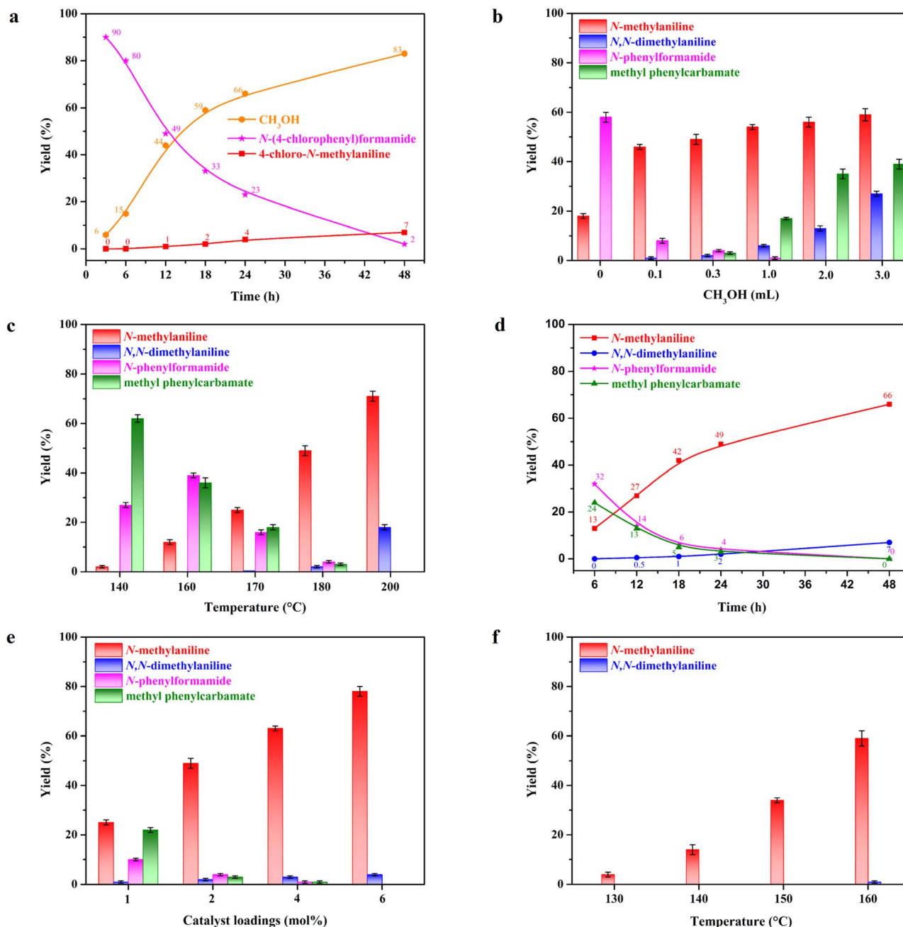
Fig. 3 Catalytic hydrogenation of 1,3-diphenylurea to N -methylaniline and N,N -dimethylaniline. Reaction conditions: 1,3-diphenylurea (2 mmol), (PPh 3 ) 3 Ir(CO)H (2 mol%), Py(CH 2 PPh 2 ) 2 (3 mol%), H 2 (30 bar), solvent (4 mL), 180 °C (bath temperature). The yield was determined by GC using biphenyl as an internal standard. Identification of the products were also confirmed by GC-MS and 1 H NMR. (a) Reaction conditions: 1,3-bis(4-chlorophenyl)urea (2 mmol), (PPh 3 ) 3 Ir(CO)H (4 mol%), Py(CH 2 PPh 2 ) 2 (5 mol%), H 2 (30 bar), 150 °C, THF (4 mL). (b) Reaction conditions: solvent (0.3 mL methanol and 3.7 mL THF), reaction temperatures (140–200 °C), reaction time (24 h). (c) Reaction conditions: solvent (0.3 mL methanol and 3.7 mL THF), reaction temperature (180 °C), reaction times (6–48 h). (d) Reaction conditions: solvent (0.3 mL methanol and 3.7 mL THF), reaction temperature (180 °C), reaction times (6–48 h). (e) Reaction conditions: 1,3-diphenylurea (2 mmol), (PPh 3 ) 3 Ir(CO)H (1–6 mol%), Py(CH 2 PPh 2 ) 2 (1.5–9 mol%), solvent (0.3 mL methanol and 3.7 mL THF), reaction temperature (180 °C), reaction time (24 h). (f) Reaction conditions: aniline (4 mmol), (PPh 3 ) 3 Ir(CO)H (1 mol%), Py(CH 2 PPh 2 ) 2 (1.5 mol%), N 2 (30 bar), solvent (0.3 mL methanol and 3.7 mL THF), reaction temperatures (130–160 °C), reaction time (20 h).
