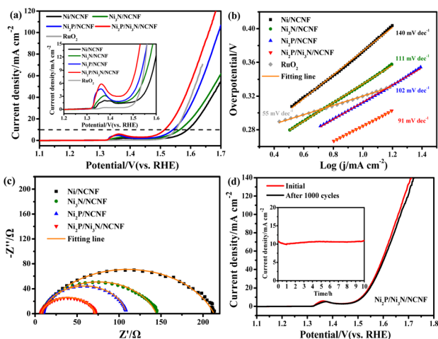
Fig. 4 (a) LSV curves and (b) Tafel slopes of all the samples. (c) EIS curves of Ni/NCNF, Ni_3N/NCNF , Ni_2P/NCNF , and Ni_2P/Ni_3N/NCNF . (d) LSV curves before and after 1000 CV cycles and the CA curve (inset in (d)) of Ni_2P/Ni_3N/NCNF in 1 M KOH solution.
