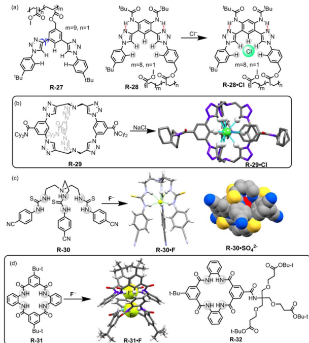
Fig. 8 (a) Chemical structures of R-27 and R-28 (blue arrows indicate the bond rotation). (b) Cl - encapsulation inside the receptor R-29. (Data from the Cambridge Crystallographic Data Centre [CCDC # 1533500]. 26 ) (c) Chemical structures of the receptors R-30 and crystal structures of R-30·F - and R-30·SO 4 2- . (Data from the Cambridge Crystallographic Data Centre [CCDC # 875998 and 875999 respectively]. 55 ) (d) Chemical structures of R-31 and 32 and crystal structure of R-31·F - . (Data from the Cambridge Crystallographic Data Centre [CCDC # 1887996]. 56 )
