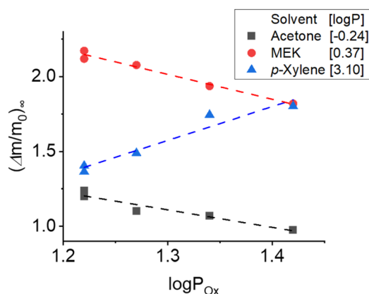
Fig. 4 Evolution of the castor oil organogels' maximum swelling capability ( \Delta m/m_0 ) _{\infty} in acetone (black), MEK (red) and p -xylene (blue) over the \log P of oligoesters O1 to O5 obtained from swelling experiments (see ESI†). Dotted lines are simply guidelines to highlight trends.
