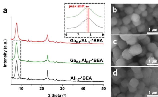
Fig. 1 (a) Powder XRD patterns of Ga 0.4 /Al 1.0 *BEA, Ga 0.4 Al 0.6 *BEA, and Al 1.0 *BEA (see also Fig. S1 of the ESI† for other samples). Inset: example of the peak shift to lower 2θ with isomorphic Ga substitution. (b–d) Scanning electron microscope (SEM) images of representative (b) Ga 0.4 /Al 1.0 *BEA, (c) Ga 0.4 Al 0.6 *BEA, and (d) Al 1.0 *BEA samples.
