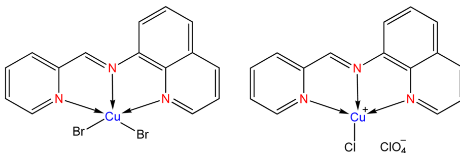
Fig. 22 Water-soluble copper(II) complexes of 2-((quinolin-8-ylimino)methyl)pyridine ligand.
