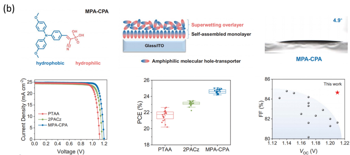
Fig. 8 (a) The molecular structures of PPA and PPAOMe and the corresponding calculated HOMO/LUMO levels. Reproduced with permission. 41 Copyright 2023, Wiley. (b) Schematic depiction of the bilayer stack of MPA-CPA molecules on an ITO-glass substrate and the corresponding device performance. Reproduced with permission. 15 Copyright 2023, AAAS.
