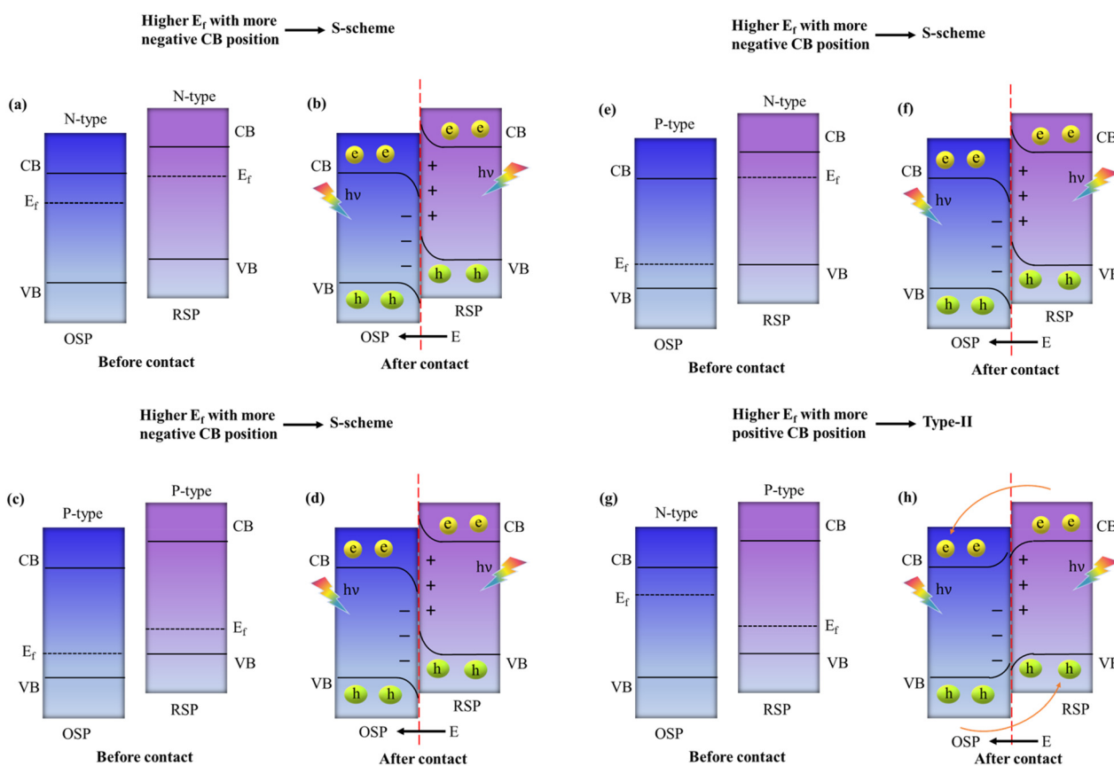
Fig. 12 Criteria for initiating (a–f) S-scheme and (g and h) type-II charge transfer mechanisms.
