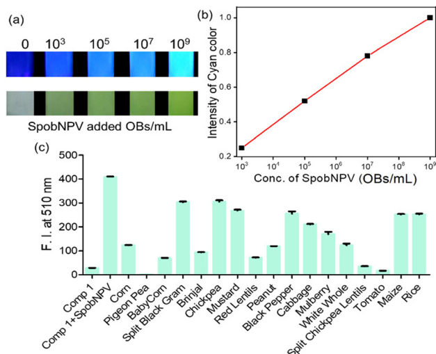
Fig. 6 (a) Changes in the color of the 1 -coated paper strips (50 μM, λ ex = 370 nm) in the presence of different concentrations of SpobNPV (seen under UV light). (b) Change in the emission color and visible color of 1 (50 μM) in the presence of different concentrations of SpobNPV. (c) Change in the emission intensity of 1 (10 μM, λ ex = 370 nm) at 510 nm in the presence of SpobNPV ( 1.3 \times 10^7 OBs mL -1 ) in different crop extracts.
