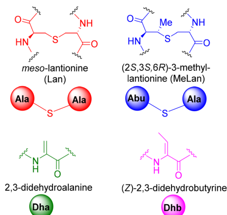
Fig. 4 Lantionine (Lan), \beta -methyl-lantionine (MeLan), dehydroalanine (Dha) and dehydrobutyrine (Dhb) notations.
