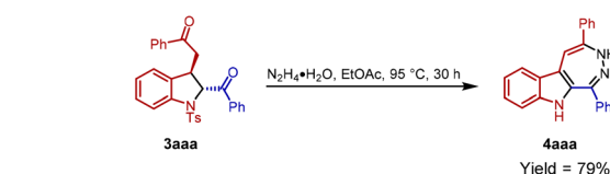
Scheme 3 Synthetic transformations.
