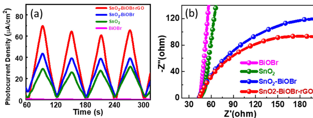
Fig. 13 (a) Photocurrent response of the SnO 2 , BiOBr, SnO 2 -BiOBr, SnO 2 -BiOBr-rGO and (b) EIS Nyquist plots under light irradiation for SnO 2 , BiOBr, SnO 2 -BiOBr, SnO 2 -BiOBr-rGO.
