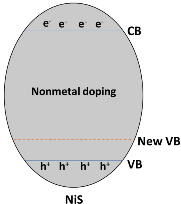
Fig. 9 Schematic illustration of the band structure modification due to non-metal doping.
