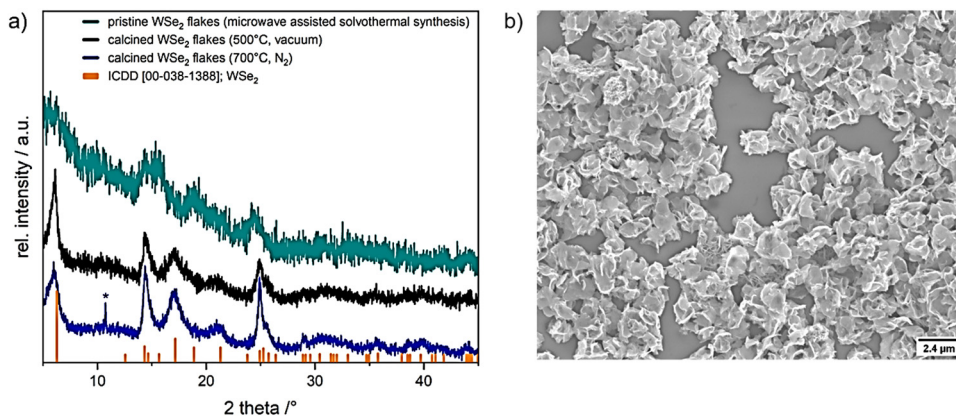
Fig. 3 (a) XRD patterns of microwave assisted solvothermal decomposition of [W\{(SeC_2H_4)_2NMe\}_2] precursor in NMP (cyan) and calcined WSe_2 flakes in vacuum at 500^\circ C (for 30 min (black)) and under nitrogen atmosphere at 700^\circ C (for 7 h (blue)), reference WSe_2 (ICDD 00-038-1388) is shown in orange, *showing a peak which could assume the formation of WO_2 (ICDD 00-082-0728, WO_2 ; Fig. S5, ESI † ). (b) SEM micrograph of resulting in WSe_2 microstructures.
