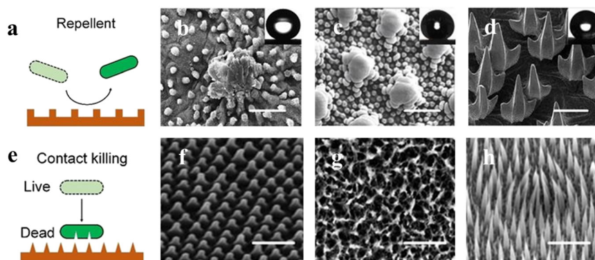
Fig. 5 Nature bacteria-repellent surface and contact-killing surfaces. (a) Graphical representation of the nature-repellent surface, (b–d) SEM images representing the microstructures on the lotus leaf (micropapilla) scalebar; 50 \mu\text{m} , springtail skin (doubly-reentrant) scalebar; 2 \mu\text{m} , and sharkskin (microdenticle) scalebar; 100 \mu\text{m} . (e) Graphical representation of the nature-contact killing surface, (f–h) SEM images representing the nanostructures on the cicada wing (nanocone) scalebar; 2 \mu\text{m} , dragonfly wing (nanopillar) scalebar; 200 nm, lizard skin (microspine) scalebar; 2.5 \mu\text{m} . 57 Copyright 2022, Multidisciplinary Digital Publishing Institute.
