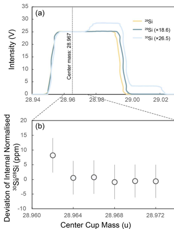
Fig. 4 (a) Mass scan of Si isotopes in a 6 \mu\text{g ml}^{-1} unspiked NSB-28 Si solution (in 0.15 \text{ mol L}^{-1} \text{ HCl} ) in medium resolution ( m/\Delta m \geq 4000 ); the measurement position of the centre cup mass is on the peak shoulder at 28.967 u. (b) Parts per million (ppm) deviation of the internally normalised ^{30}\text{Si}/^{28}\text{Si} for the mass range from 28.962 to 28.972 u of the centre cup mass.
