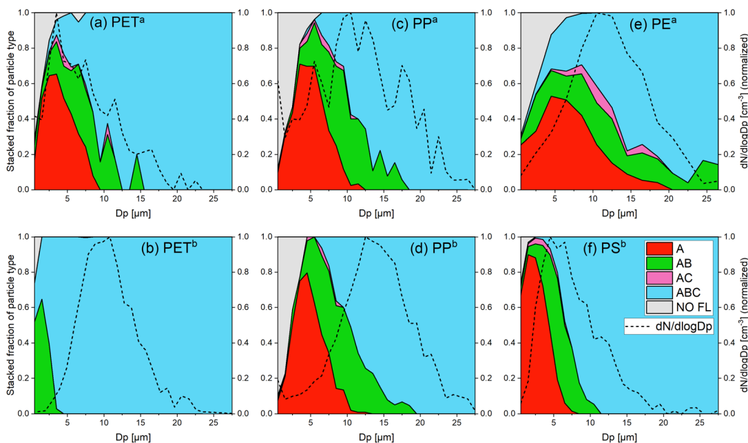
Fig. 1 Stacked fraction of the fluorescent particle types and size distribution of all detected particles for (a) PET a , (b) PET b , (c) PP a , (d) PP b , (e) PE a and (f) PS b . These graphs show the proportion of each particle type (A, AB, AC, ABC and NO FL) in all measured particles of a certain size D_p . The size distributions ( dN/d\log D_p ) were normalized (the maximum was set to 1). The colors refer to the particle types according to the classification in Fig. 4. The gray area shows the fraction of non-fluorescent particles. The line under the gray area is the detection effectivity. For all samples, fluorescence emission on a single particle level could be detected for most of the particles. There is a general trend of channel evolution with the particle size of A \rightarrow AB \rightarrow ABC and a few AC particles. Other particle types (e.g. B, C and BC) were not recorded.
