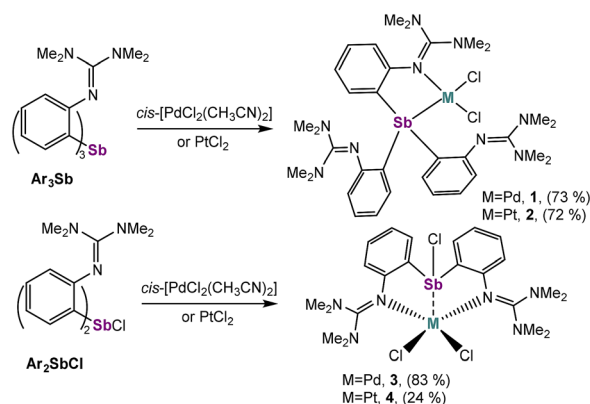
Scheme 1 Synthesis of the investigated complexes.
